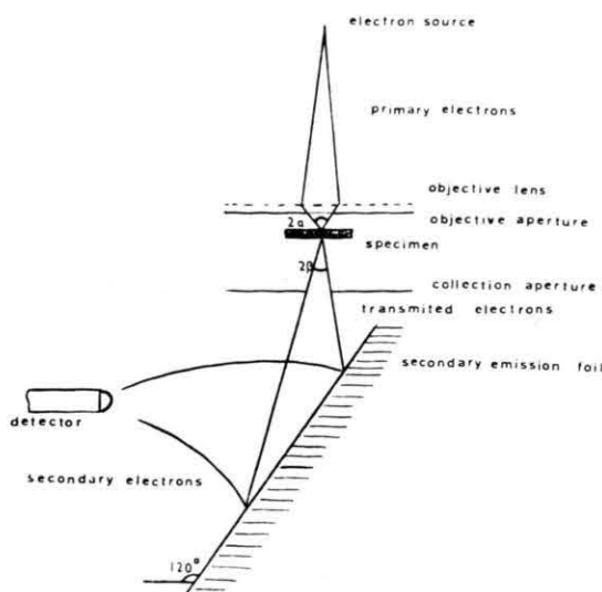
Fig. 1. Transmission — detection device.
